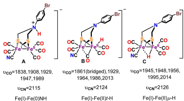
Fig. 10 Probable one electron reduced species and their computed \nu_{\text{CO}} and \nu_{\text{CN}} vibrational frequencies.
