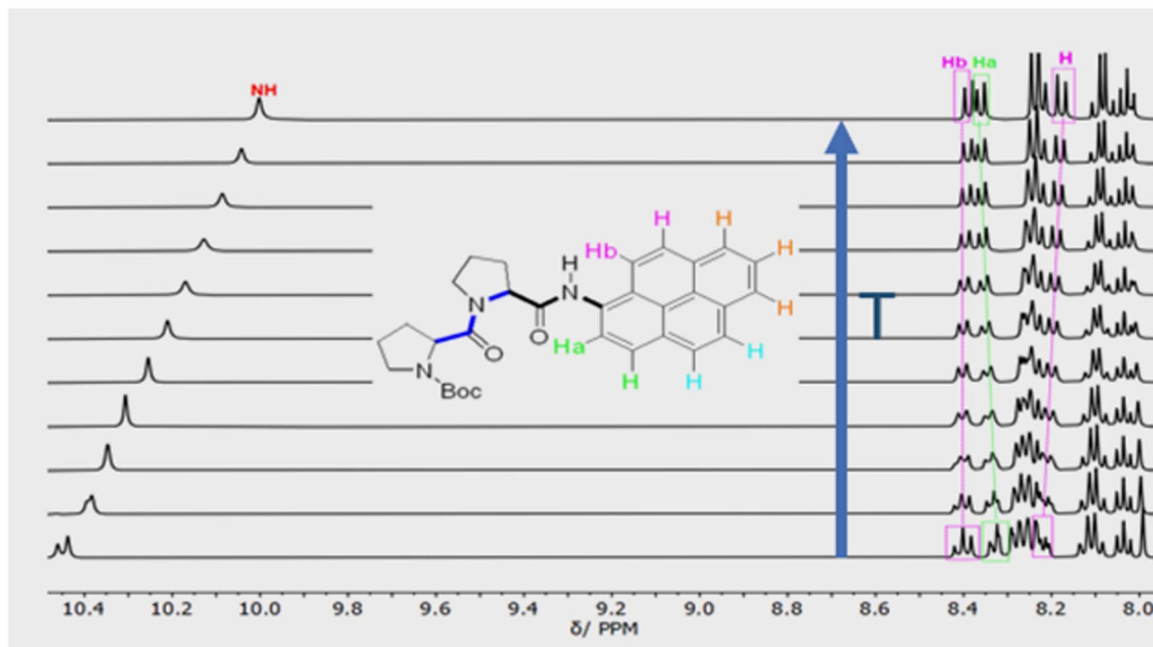
Fig. 3 Variable temperature ^1\text{H} NMR spectra of PY-P 2 in D_6 -DMSO showing the aromatic region and the most downfield proton resonances. The blue arrow indicates the direction of increasing temperature. The first spectrum was recorded at 298 K, the second at 313 K and subsequent spectra were recorded at intervals of 10 K until 403 K.
