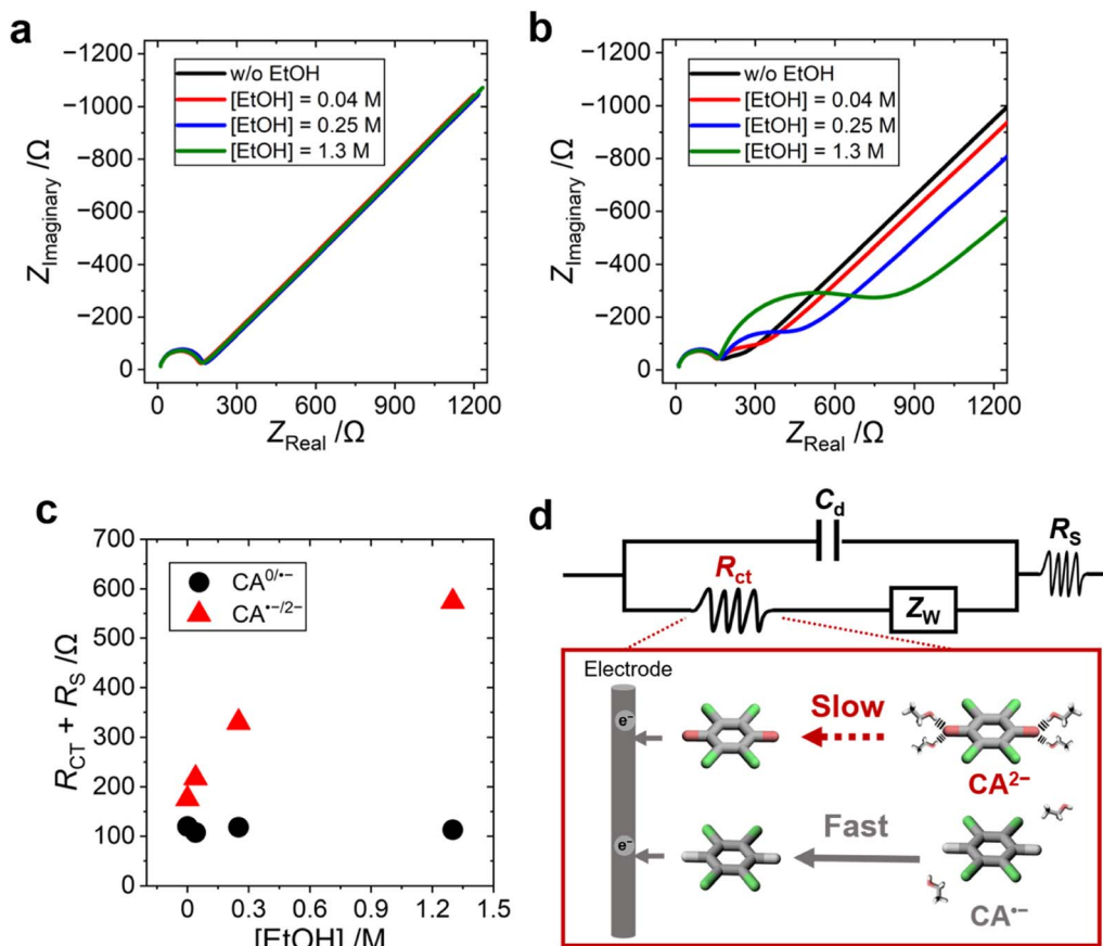
Fig. 4 (a and b) Nyquist plots of (a) \text{CA}/\text{CA}^{\bullet-} and (b) \text{CA}^{\bullet-}/\text{CA}^{2-} redox pairs and (c) the sum of the solution resistance ( R_{\text{s}} ) and charge transfer resistance ( R_{\text{ct}} ) in acetonitrile with various EtOH concentrations. (d) The equivalent circuit and schematics showing the charge-transfer processes of \text{CA}^{\bullet-} and \text{CA}^{2-} near the electrode surface, and dissociation of EtOH from \text{CA}^{2-} increases the R_{\text{ct}} . [\text{CA}] = 1.0 \text{ mM} , [\text{TBAPF}_6] = 0.1 \text{ M} , and [\text{EtOH}] = 0, 0.040, 0.25, \text{ and } 1.3 \text{ M} .
