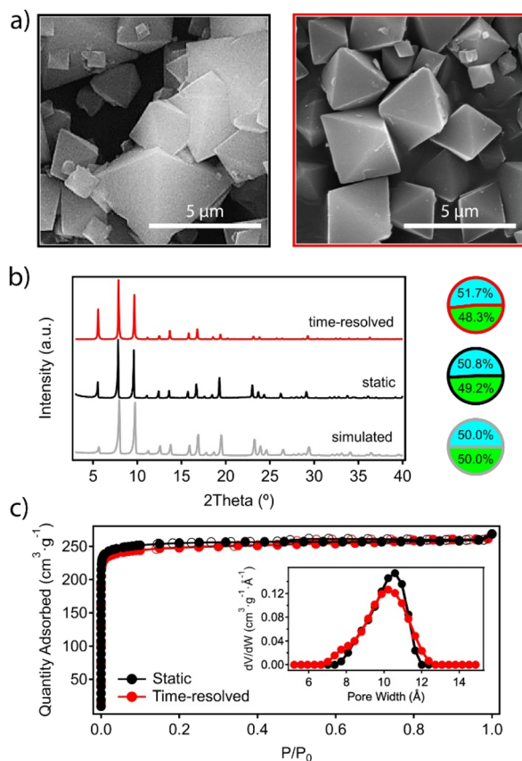
Fig. 3 (a) SEM micrographs of MUV-10 crystals prepared by the static (left) and time-resolved (right) methods. (b) Comparison of their PXRD patterns and metal ratios with those expected for an ideal framework. (c) \text{N}_2 isotherms and PSD plots at 77 K.
