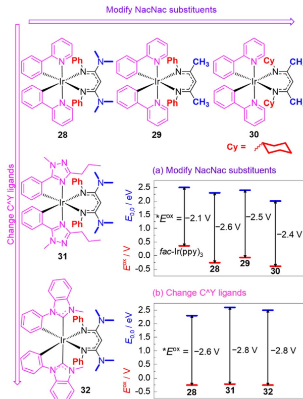
Fig. 12 Summary of representative Ir(C ^ Y) 2 (NacNac) photosensitizers, demonstrating structure–property relationships involving E^{\text{ox}} (red lines) and E_{0,0} (blue lines). The E^{\text{ox}} values are referenced to the ferrocene couple, and the vertical arrows represent the absolute value of *E^{\text{ox}} , as per eqn (1).
