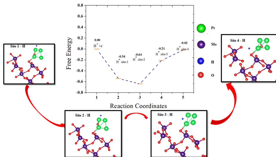
Fig. 8 Schematic presentation of a free energy diagram for the HER on the surface of Pt@MoO 3 (011). Optimized H* adsorption structures from site 1 to site 4 at different locations on Pt@MoO 3 (011) are shown in the black boxes according to the red arrows.
