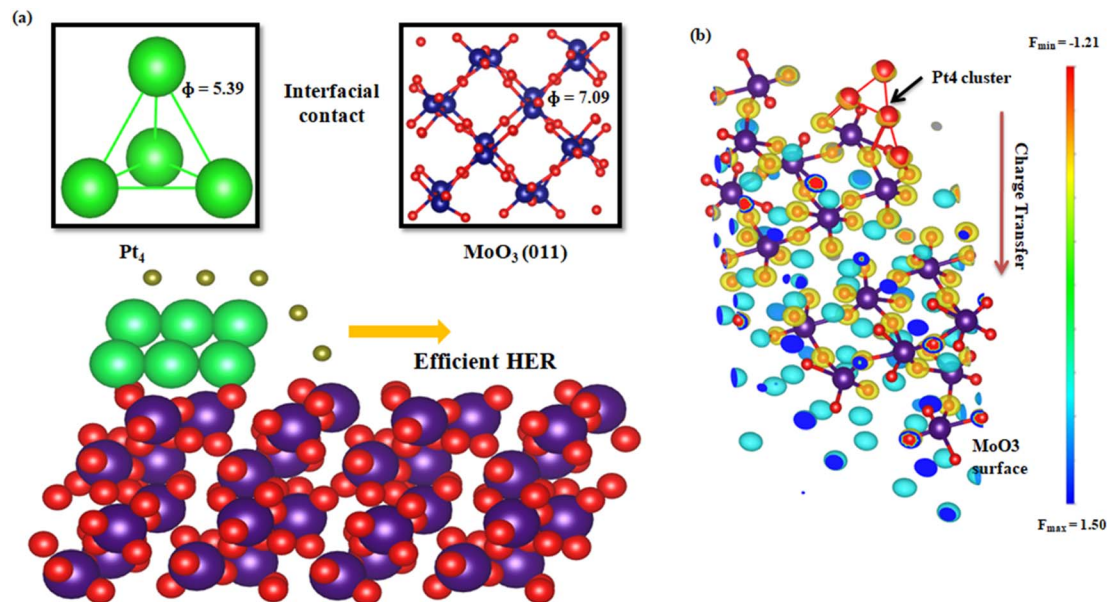
Fig. 7 (a) Schematic illustration of the hydrogen spillover mechanism over a Pt 4 @MoO 3 (011) surface. (b) Charge density difference plot across the Pt 4 @MoO 3 (011) surface.
