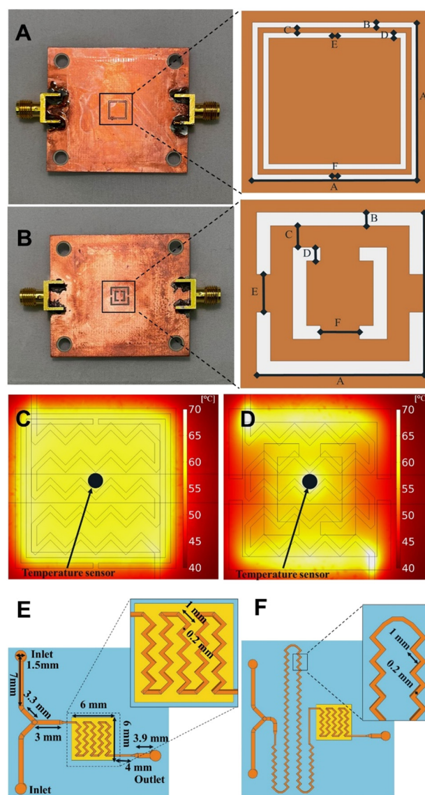
Fig. 1 A) 2 GHz CSRR. B) 8 GHz CSRR. C) COMSOL MW heating simulation with input power of 1 W at 2 GHz. D) COMSOL MW heating simulation with input power of 1 W at 8 GHz. E) Flow cell A. F) Flow cell B.
