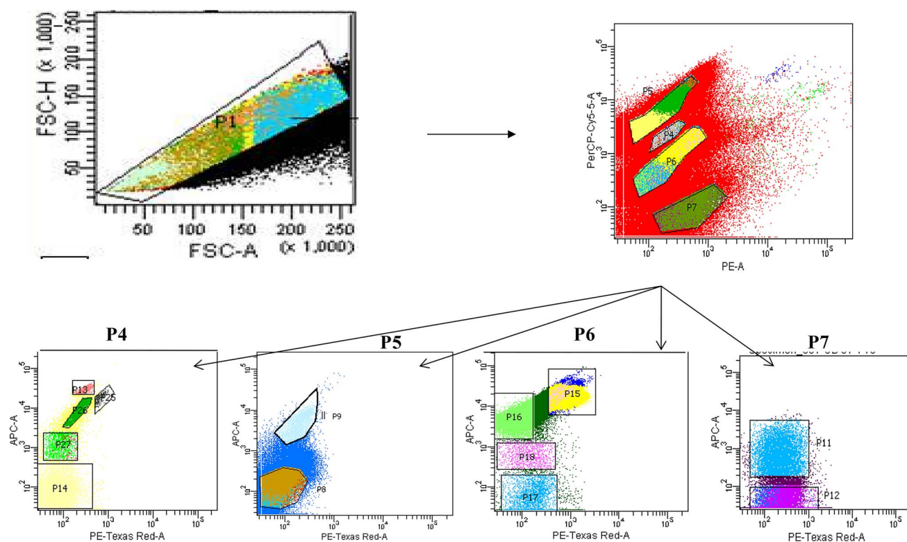
Fig. 2 Bivariate scatter plots analyzed using FACS sort flow cytometry, showing gating of phytoplankton population based on pigment auto-fluorescence and their cell size. P7 refers to the summer data also presented in Fig. 7.
