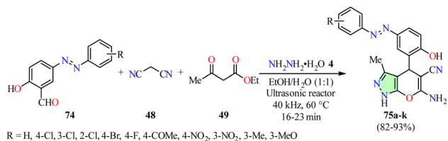
Scheme 21 Synthesis and anticancer evaluation of 1,4-dihydropyrano [2,3- c ]pyrazole-5-carbonitriles 75 .
