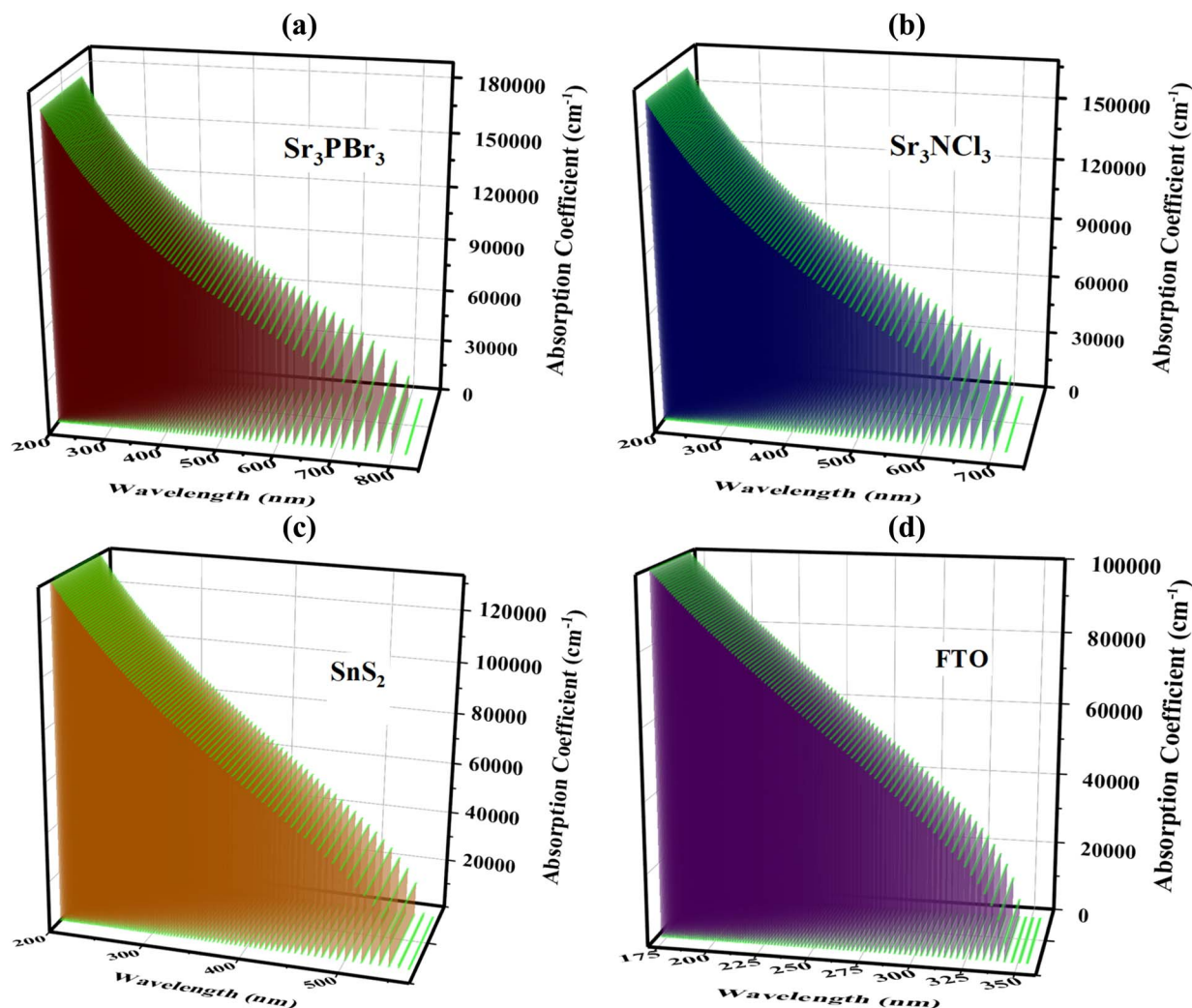
Fig. 12 An analysis of the absorption coefficient is conducted for the ideal SC architecture of FTO/ \text{SnS}_2 / \text{Sr}_3\text{PBr}_3 / \text{Sr}_3\text{NCl}_3 /Ni, specifically for the materials: (a) \text{Sr}_3\text{PBr}_3 , (b) \text{Sr}_3\text{NCl}_3 , (c) \text{SnS}_2 , and (d) FTO.
