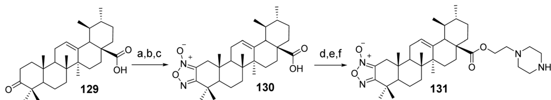
(a) Isoamyl nitrite, t-BuOK, t-BuOH, rt, 2.5 h; (b) Hydroxylamine hydrochloride, Pyridine, 110 °C, 2 h; (c) EtOH, NaOH, NaOCl, rt, 2 min; (d) 2-chloroethanol, K 2 CO 3 , DMF, 60 °C, 3 h; (e) MsCl, Pyridine, 10 °C~rt, 3 h; (f) Piperazine, K 2 CO 3 , DMF, 60 °C, 30 min.
