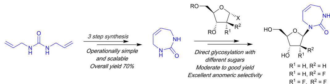
Scheme 1 Strategies for the synthesis of 1,3-diazepinone and 2'-deoxyribo and 2'-fluorinated diazepinone nucleosides.
