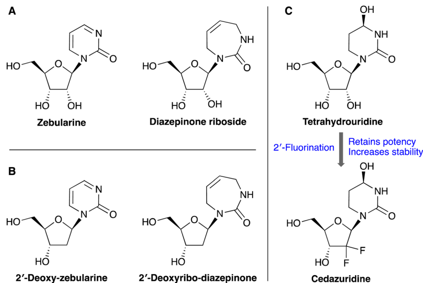
Fig. 1 Example of chemically modified cytidine analogues: (A) ribose-based nucleoside inhibitors of cytidine deaminase (CDA). (B) Corresponding 2'-deoxy analogues which inhibit APOBEC3 enzymes when incorporated into oligonucleotides. (C) 2'-Fluorination has successfully been used to increase the stability of CDA inhibitors.
