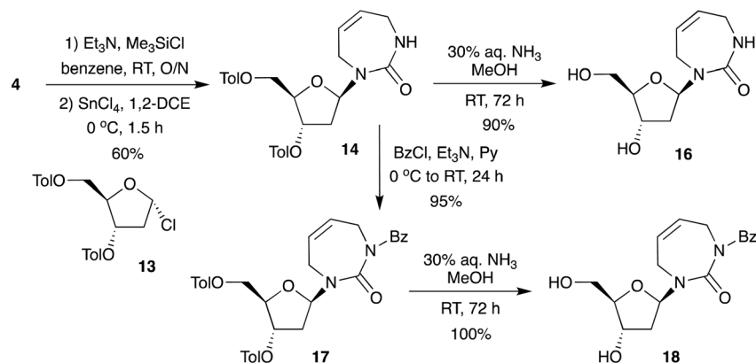
Scheme 4 Synthesis of 2'-deoxyribo-diazepinone nucleoside by direct glycosylation.
