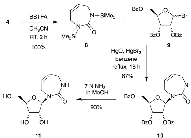
Scheme 3 Synthesis of diazepinone riboside.
