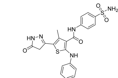
4-Methyl-5-(5-oxo-4,5-dihydro-1H-pyrazol-3-yl)-2-(phenylamino)-N-(4-sulfamoylphenyl)thiophene-3-carboxamide
