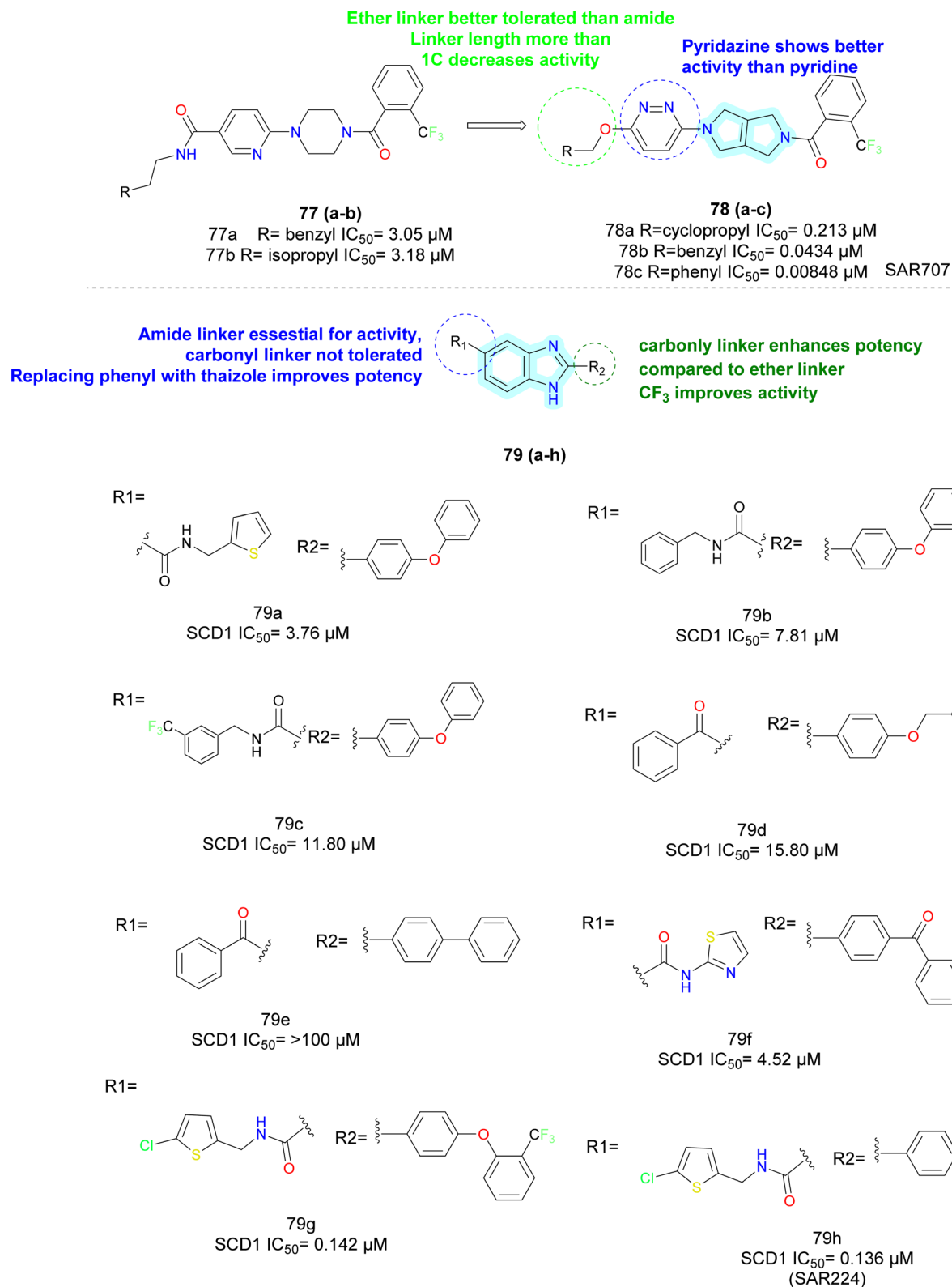
Fig. 12 Bicyclic SCD1 inhibitors: development of SAR 707 and SAR 224.
