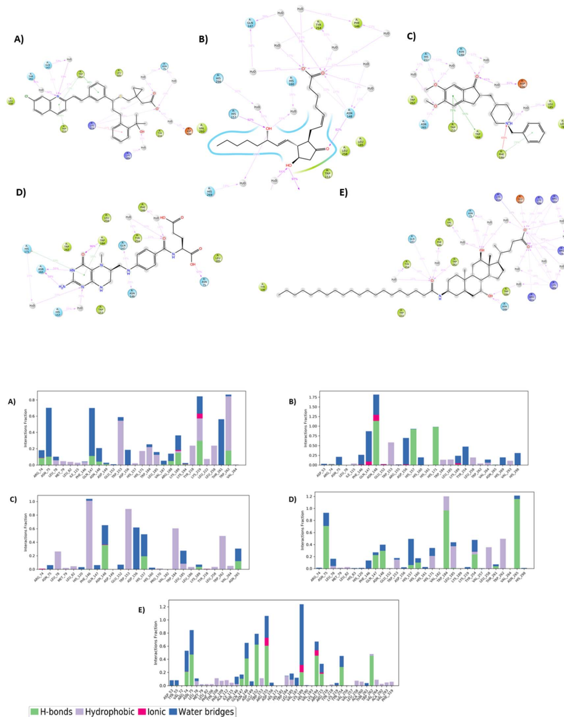
Fig. 3 (A) 2D amino acid residue interaction diagrams of ligands after molecular dynamics stimulation (A-Montelukast, B-Dinoprostone, C-Donepezil, D-Levomefolic acid, E-Aramchol). (B) Protein ligand contact plot of the ligands (A-Montelukast, B-Dinoprostone, C-Donepezil, D-Levomefolic acid, E-Aramchol).
