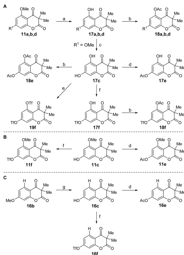
Scheme 2 Derivatization of chromene diones by selective O -demethylation, O -acetylation and O -triflation starting from 11a,b,d (A), 11c (B), 16b (C), respectively. Reagents and conditions: (a) BBr 3 (1.1–2.5 eq.), DCM, -78^{\circ}\text{C} ( 11d ) or 0^{\circ}\text{C} ( 11a,b ) to rt, 20 h. (b) Ac 2 O (135–200 eq.), pyridine (160–235 eq.), DCM, rt, 21 h. (c) BBr 3 (5.0 eq.), DCM, 0 to 40^{\circ}\text{C} , 3 d. (d) Ac 2 O (1.05–1.1 eq.), pyridine (1.05–1.5 eq.), DCM, rt, 17–20 h. (e) Tf 2 O (2.2 eq.), pyridine (2.2 eq.), DCM, 0^{\circ}\text{C} to rt, 4.5 h. (f) Tf 2 O (1.05–1.1 eq.), pyridine (1.05–1.5 eq.), DCM, 0^{\circ}\text{C} to rt, 4.5 h. (g) BBr 3 (3.5 eq.), DCM, -78^{\circ}\text{C} to rt, 7 d.
