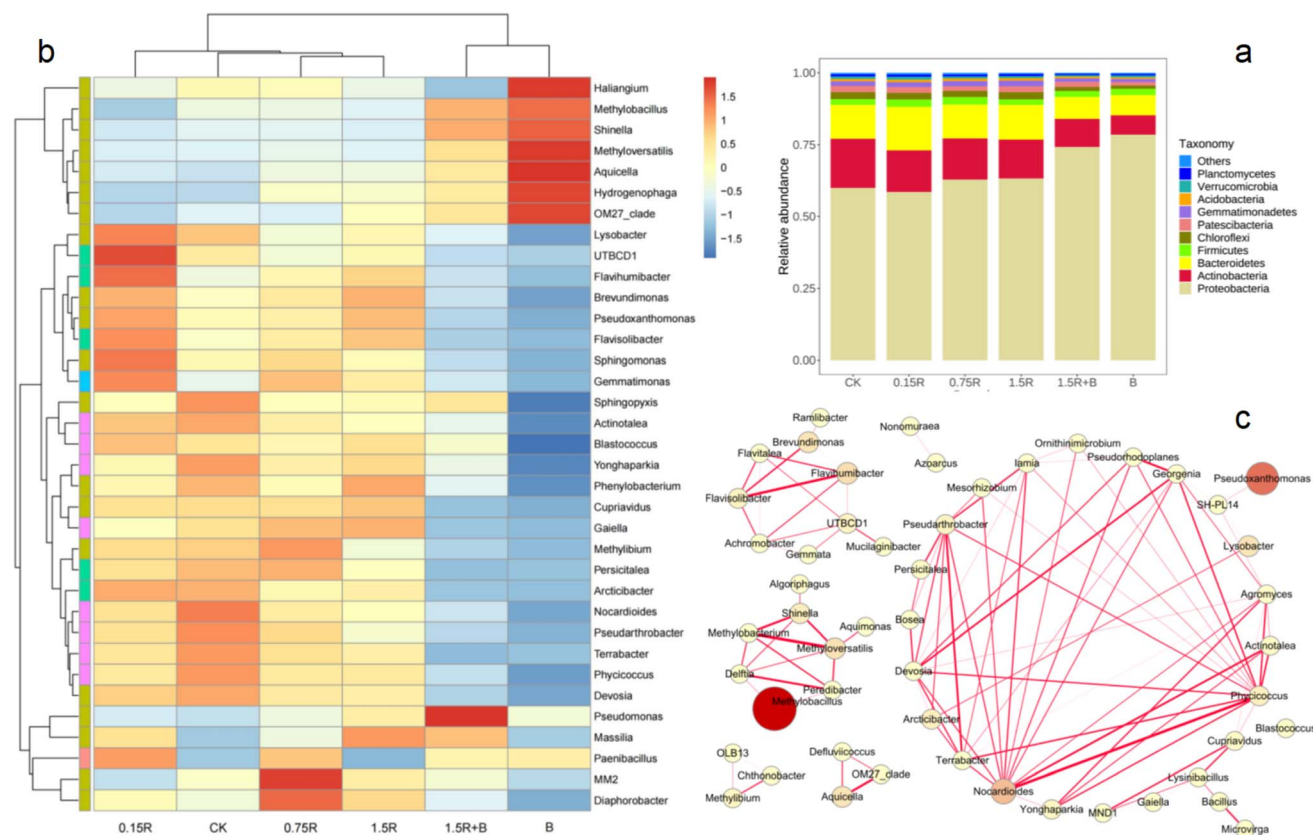
Fig. 4 Soil microbial species distributions and interspecies relationships after 15 days of treatment. (a) Histogram of the relative abundance of species at the phylum level. (b) Cluster map of species-level species distributions. (c) Visualization of microbial genus-level correlations. CK: the control treatment without strain C1 or resveratrol; 0.15R, 0.75R, and 1.5R represent the treatments with 0.15 mg L -1 , 0.75 mg L -1 and 1.5 mg L -1 resveratrol, respectively, but without strain C1; 1.5R + B: the treatments with both 1.5 mg L -1 resveratrol and strain C1; B: the treatments with strain C1 but without resveratrol.
