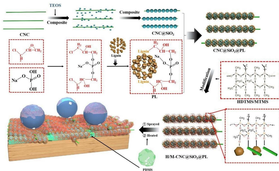
Fig. 18 Scheme for preparation of superhydrophobic coatings using cellulose nanocrystals (CNC)– \text{SiO}_2 –phosphorylated lignin (PL) rods. 113 Reproduced from ref. 113 with permission from Polymers , copyright 2023.
