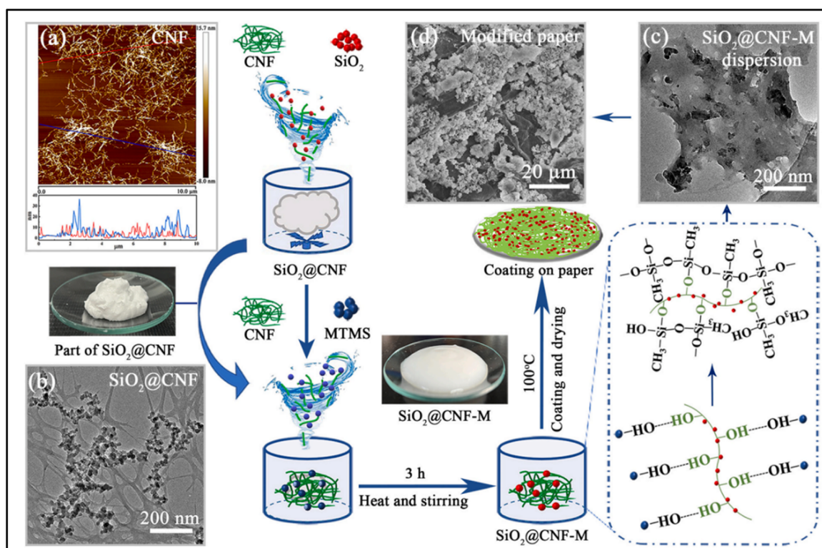
Fig. 19 Schematic representation of fabricating \text{SiO}_2 @CNF-M water dispersion and the coating. (a) The AFM morphology of CNF. (b) The \text{SiO}_2 @CNF and (c) \text{SiO}_2 @CNF-M dispersion's TEM morphology. (d) \text{SiO}_2 @CNF-M coated on paper SEM morphology. 115 Reproduced from ref. 115 with permission from Carbohydrate Polymers , copyright 2022.
