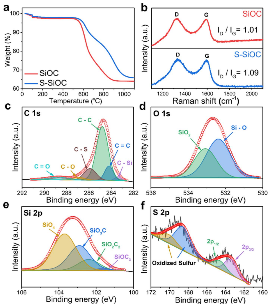
Fig. 2 (a) TGA curves of SiOC and S-SiOC at a heating rate of 5\text{ }^\circ\text{C min}^{-1} under the air atmosphere. (b) Raman spectra of SiOC and S-SiOC. High resolution XPS spectra of (c) C 1s, (d) O 1s, (e) Si 2p, (f) S 2p in S-SiOC.
