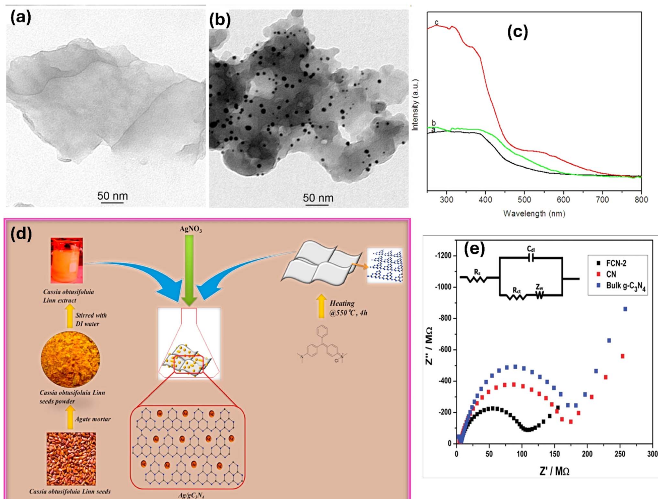
Fig. 2 Tem image of (a) \text{g-C}_3\text{N}_4 , (b) Au/ \text{g-C}_3\text{N}_4 , (c) DRS data of \text{g-C}_3\text{N}_4 nanosheets, bulk \text{g-C}_3\text{N}_4 , and AuNP/ \text{g-C}_3\text{N}_4 nanohybrids reprinted with the permission of ref. 72, copyright 2024, American Chemical Society; (d) synthesis of Ag/ \text{g-C}_3\text{N}_4 via green route, reprinted with the permission of ref. 73, copyright 2024, Elsevier; and (e) EIS of the \text{g-C}_3\text{N}_4 , and pure and Fe-doped \text{g-C}_3\text{N}_4 nanosheets, reprinted with the permission of ref. 74, copyright 2024, RSC.
