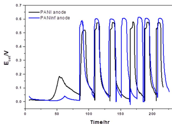
Fig. 3 Charge-discharge curves of MFCs with PANI (black) and PANInf (blue) anodes.
