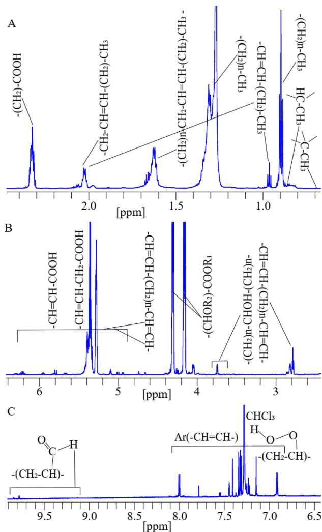
Fig. 2 A representative 1D\ ^1H -NMR spectrum assigned with functional groups of lipids at their corresponding chemical shifts of a cheese sample dissolved in deuterated chloroform. 79,80
