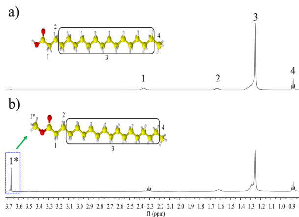
Fig. 1 1 H NMR spectra: (a) stearic acid (SA) used as a reagent in the esterification reaction, and (b) methyl stearate (MST) produced in the reaction of SA with methanol.
