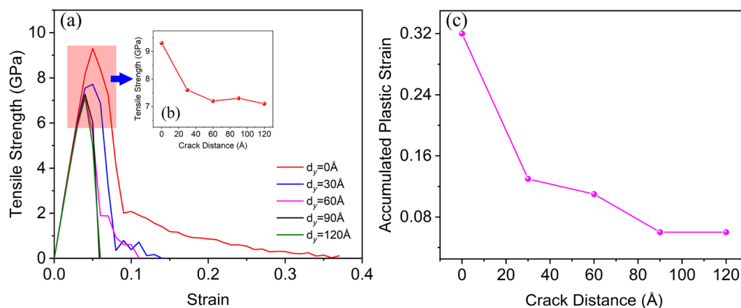
Fig. 3 Stress–strain behaviors of tensile model with various distances between two cracks in the Y-direction: (a) stress–strain curve, and the inset (b) denote the tensile strength of different model, and (c) accumulated plastic strain of tensile model.
