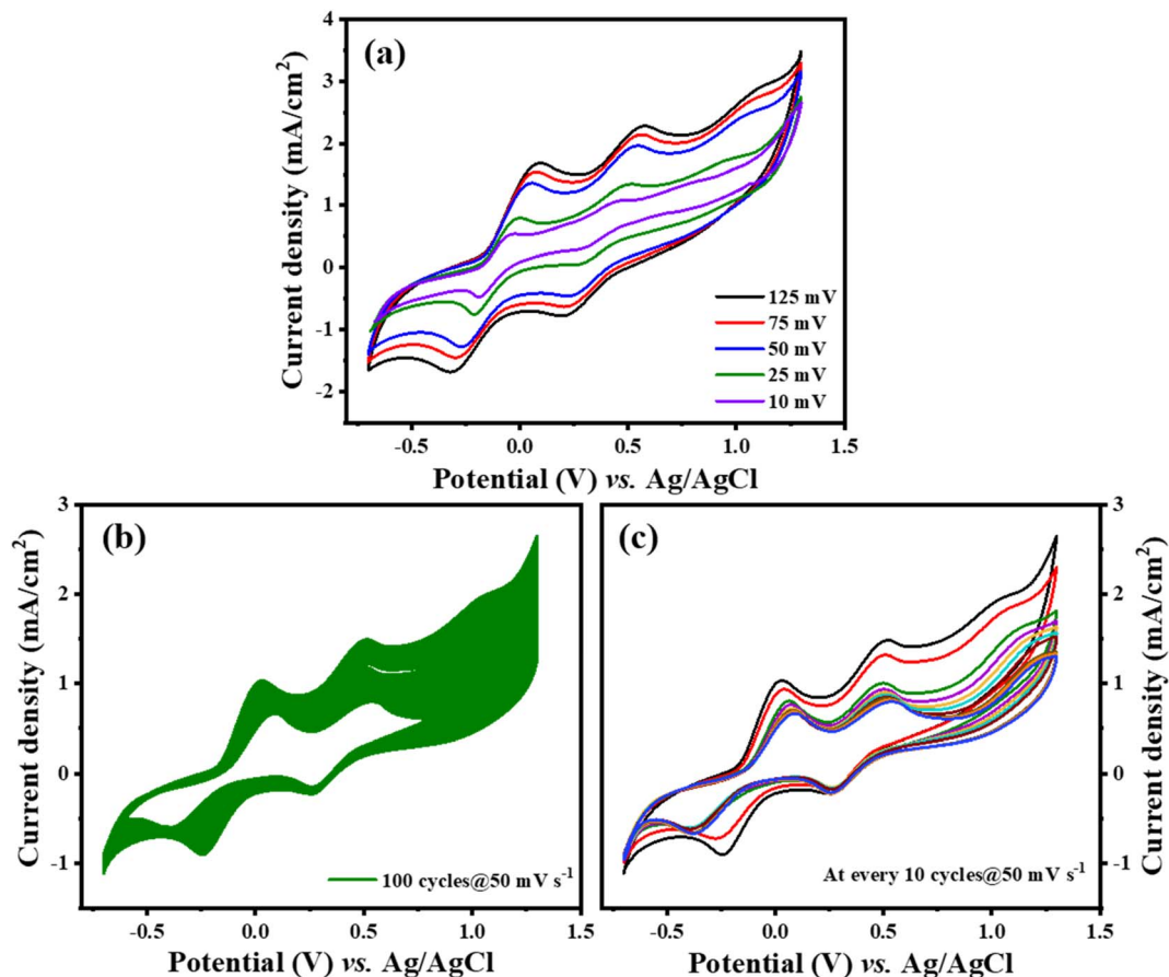
Fig. 6 (a) \text{Ti}_3\text{C}_2\text{T}_x\text{-PTh} at various scan rates (b) and (c) stability test of \text{Ti}_3\text{C}_2\text{T}_x\text{-PTh} at 50 mV \text{s}^{-1} for 100 cycles and plotted at every 10 cycles.
