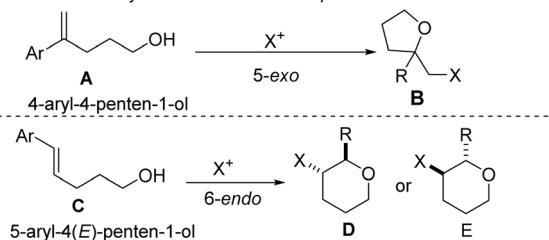
Fig. 2 (A) Prior cyclizations utilizing lactam-tethered alkenol 1 , (B) proposed plan for accessing lactam-fused bromotetrahydropyrans from 1 , (C) reported predictive approaches for halo-cycloetherification of simple alkenols.
