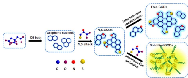
Fig. 5 Synthetic strategy for the preparation of N–S co-doped GQDs. Reproduced with permission from ref. 122. Copyright © Elsevier, 2017.
