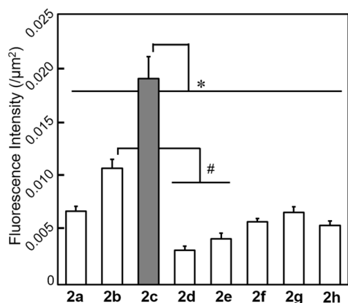
Fig. 4 Intracellular fluorescence intensity of HeLa cells incubated with 2 (2 \mu M) for 30 min at 37 ^{\circ} C detected by CLSM. Mean \pm SE, n = 39–40, * p < 0.05 relative to 2c , # p < 0.05 relative to 2b (Tukey–Kramer's test).
