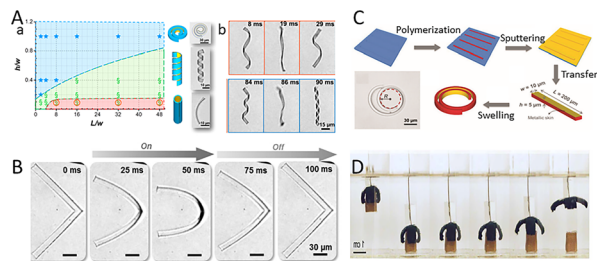
Fig. 2 (A) The shape of the double-layer hydrogel bands with different sections and lengths, and the unwinding and reversal of the helix can be completed within 90 milliseconds (this figure has been reproduced from ref. 34 with permission from ACS Publications, copyright 2024). (B) Various states of L-type microgels in a modulation cycle (this figure has been reproduced from ref. 35 with permission from Wiley-VCH, copyright 2024). (C) Preparation of bilayer spiral microhydrogels (this figure has been reproduced from ref. 37 with permission from John Wiley and Sons, copyright 2024). (D) Grasping objects using soft micro-robots made with a PVA passivation layer (this figure has been reproduced from ref. 36 with permission from Science Robotics, copyright 2024).
