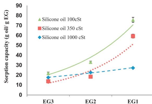
Fig. 14 The oil sorption capacities of EGs prepared at different expansion temperatures. Reprinted with permission from ref. 72.
