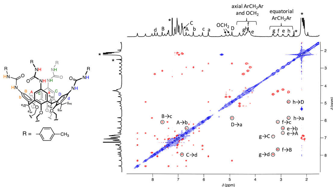
Fig. 3 ROESY NMR spectrum (500 MHz, \text{CDCl}_3/\text{DMSO}-d_6 98 : 2, 298 K) of [\text{UC4T}] = 1 mM. The asterisks indicate the residual peaks of the solvents. The labels of the assigned NMR signals are shown in the schematic drawing of UC4T on the left.
