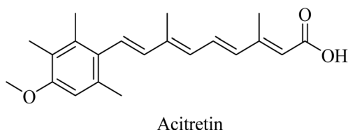
Fig. 35 The chemical structure of acitretin.
