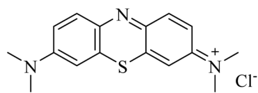
Methylthioninium chloride
