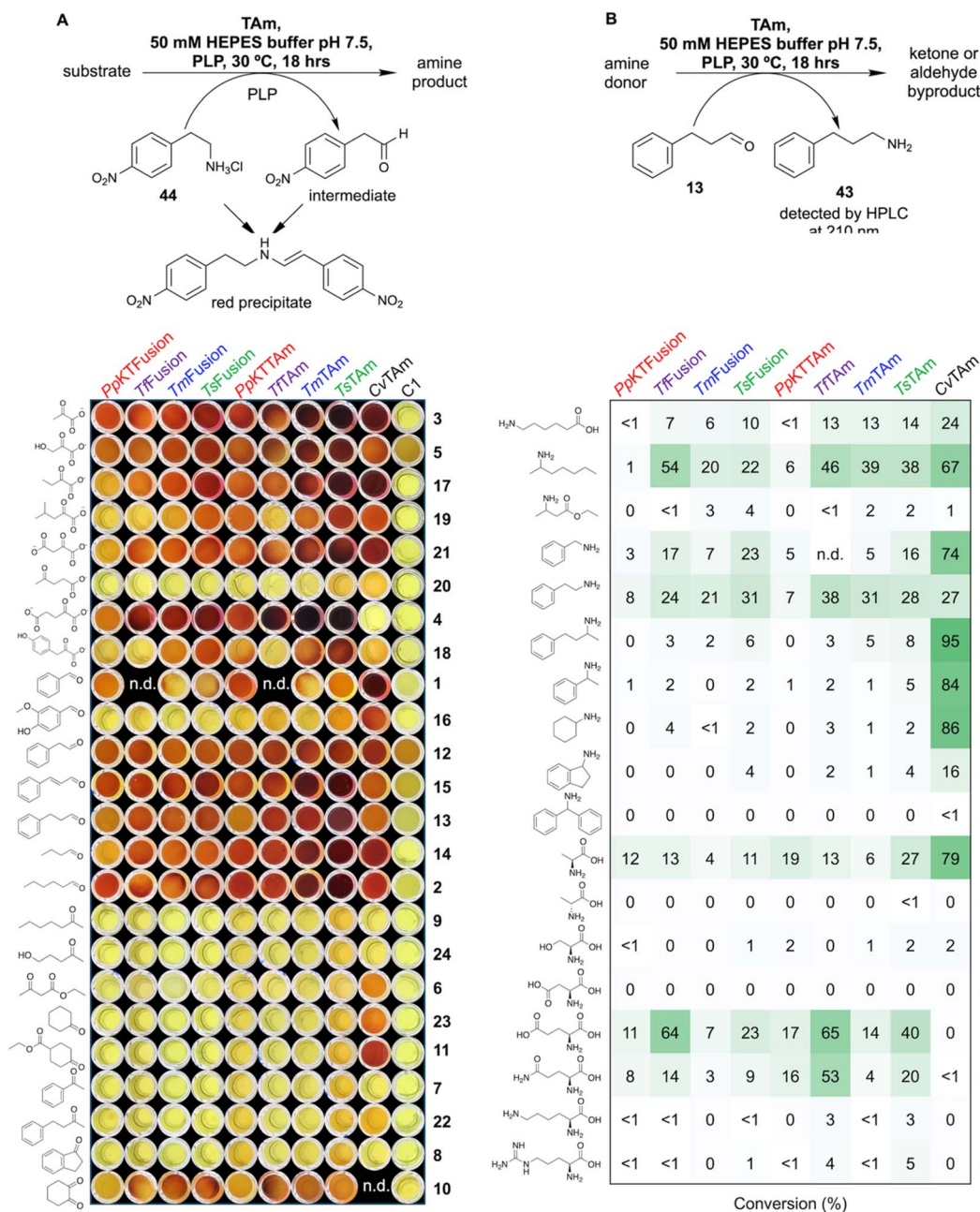
Fig. 6 Transaminase activity screening of PpKTFusion, TFusion, TmFusion, TsFusion, PpKTAm, TmTAm, TsTAm, alongside CvTAm control using 1–44. (A) Colorimetric assays with \alpha -keto acids, aldehydes, and ketones employing 44 as an amine donor and shown with no enzyme (C1) control. Reactions were performed in triplicate or duplicate and contained 50 mM HEPES buffer at pH 7.5, 25 mM 44, 1.0 mM PLP, and a substrate at 10 mM. Reactions were initiated by the addition of enzyme (0.01 mg mL -1 final concentration) and run at 30 °C for 18 hours. The dark red colouration in samples indicates conversion levels \geq 20\% . (B) Conversions with various amine donors using 13 as a substrate. Assays were prepared with 25 mM amine donor, 10 mM 13, 1.0 mM PLP, and purified enzyme at 0.05 mg mL -1 and were performed in duplicate. Percentage conversions were determined using 43 yield detected at 210 nm by HPLC. Assays were run alongside no enzyme controls, and any background (if present) was subtracted from the reactions. Values shown are the mean of two measurements, with SD < 10%.
