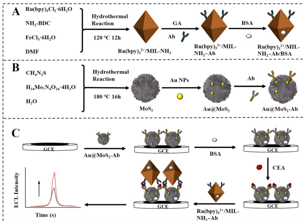
Fig. 5 Synthesis of (A) \text{Ru}(\text{bpy})_3^{2+}/\text{MIL-NH}_2\text{-Ab} bioconjugates and (B) \text{Ab-Au@MoS}_2 , as well as (C) the assembly procedure of the suggested triple improved ECL immunosensor. Reproduced from ref. 54 with permission from [Elsevier], copyright [2024].
