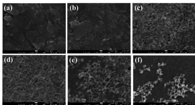
Fig. 8 SEM images of the membranes fouled by the feed water (a) without pretreatment, and pretreated by (b) UV, (c) Fe(vi), (d) UV/Fe(vi)-1, (e) UV/Fe(vi)-2, and (f) UV/Fe(vi)-3 (500 00 \times magnification).
