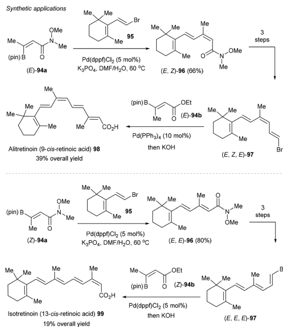
Scheme 37 Synthetic applications.
