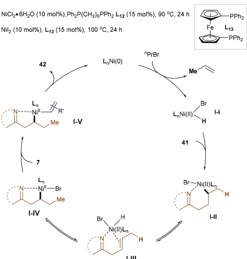
Scheme 13 Ni(II)H-catalyzed \beta -vinylation.
