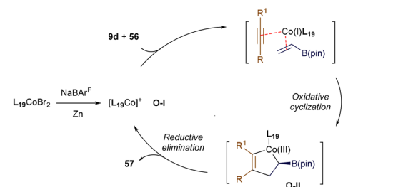
Scheme 21 Co(I)-catalyzed [2 + 2] cycloaddition.
