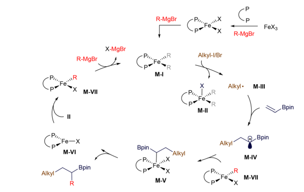
Scheme 20 ATRA reaction.
