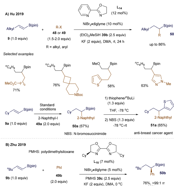
Scheme 16 NiH-catalyzed hydrocarbonation.
