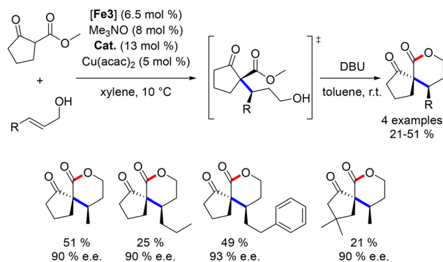
Scheme 76 Synthesis of γ-lactones.
