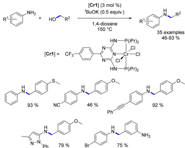
Scheme 53 Chromium-catalysed alkylation of anilines.
