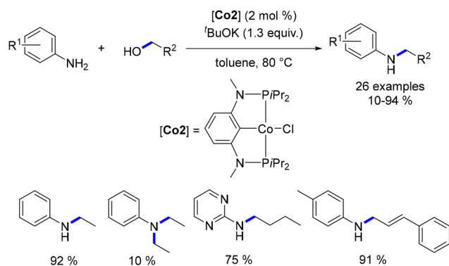
Scheme 35 Cobalt-catalysed alkylation of anilines, as reported by Kirchner.
