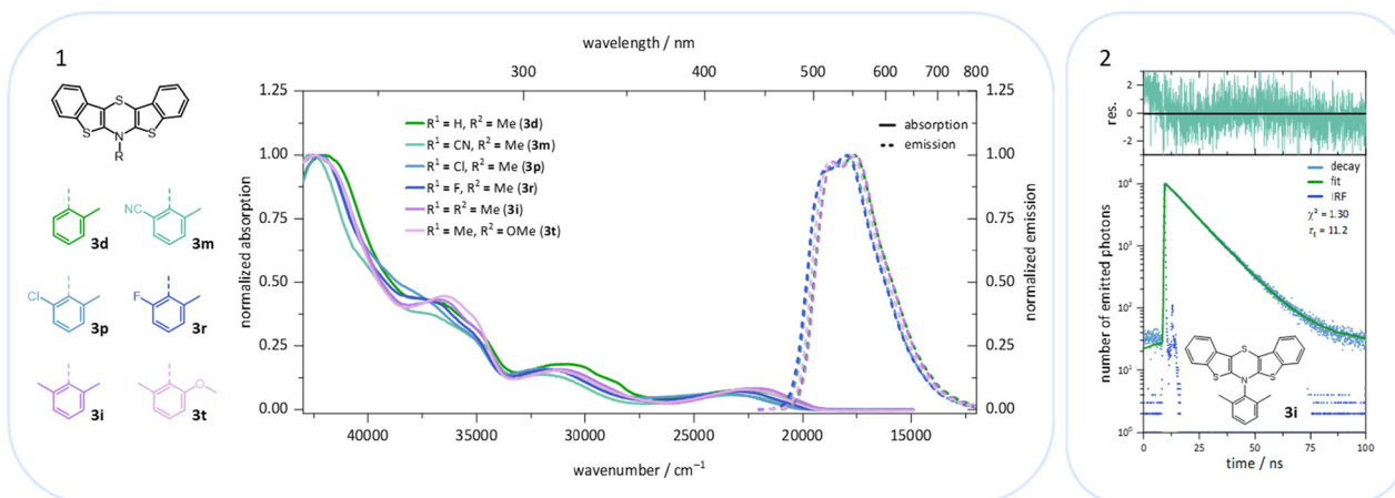
Fig. 11 (1) UV/vis absorption and emission spectra of BBTBs 3 in solution (recorded in \text{CH}_2\text{Cl}_2 , T = 298 \text{ K} , c = 10^{-5} to 10^{-7} \text{ M} ). (2) Lifetime data measured by TCSPC experiments exemplarily given for 3i .
