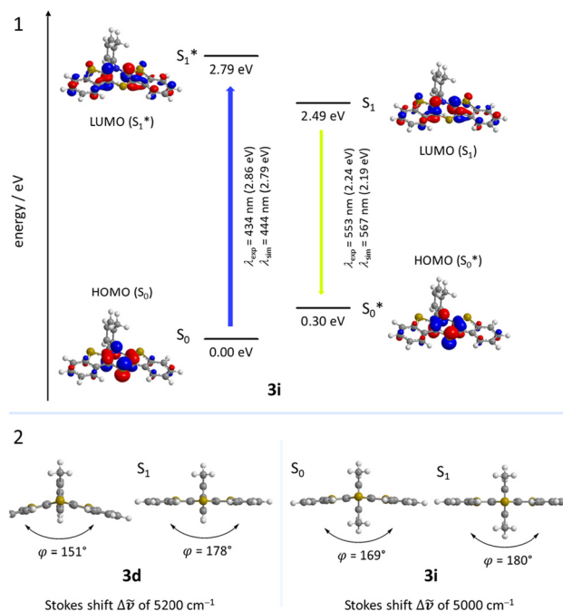
Fig. 13 (1) TD-DFT calculated Jabłoński diagram of BTT 3i with the associated Kohn–Sham frontier orbitals of the S_0 – S_1^* -transition and S_0^* – S_1 -transition. (2) Vibrational relaxed minimum S_0 - and S_1 -geometries of 3d and 3i indicated with their S,N -folding angles \phi and Stokes shifts \Delta\tilde{\nu} (PBE1PBE/6-311++G**, IEFPCM \text{CH}_2\text{Cl}_2 , isosurface value 0.05 a.u.).
