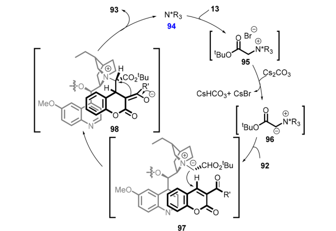
Scheme 18 (DHQ)_2P\text{YR} catalyzed enantioselective MIRC cyclopropanation of coumarins.
