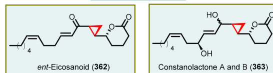
Scheme 81 Chiral Rh(III) complex-catalyzed cyclopropanation of N -enoxypthalimides and electron-deficient olefins.
