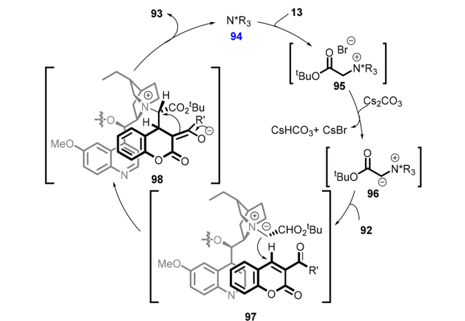
Scheme 18 (\text{DHQ})_2\text{PYR} catalyzed enantioselective MIRC cyclopropanation of coumarins.
