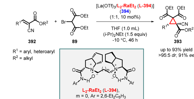
Scheme 87 N,N' -Dioxide-lanthanum(III) complex catalyzed enantioselective MIRC cyclopropanation.
