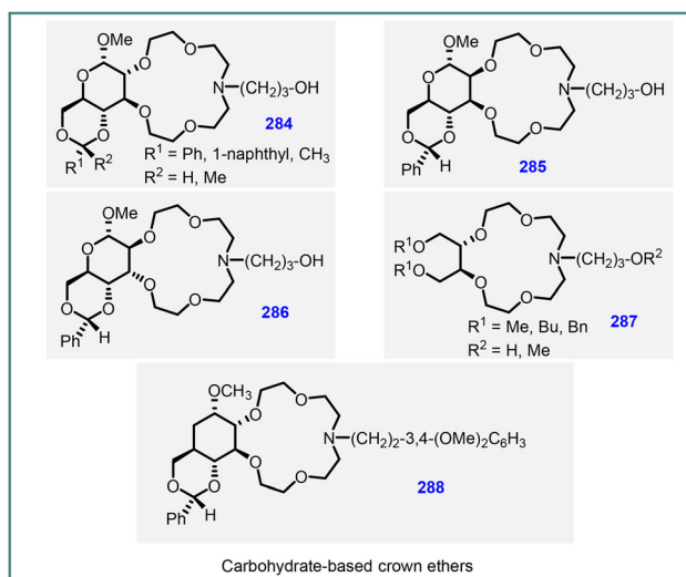
Scheme 65 MIRC cyclopropanation using chiral \alpha -D-glucopyranoside-based crown ether.
