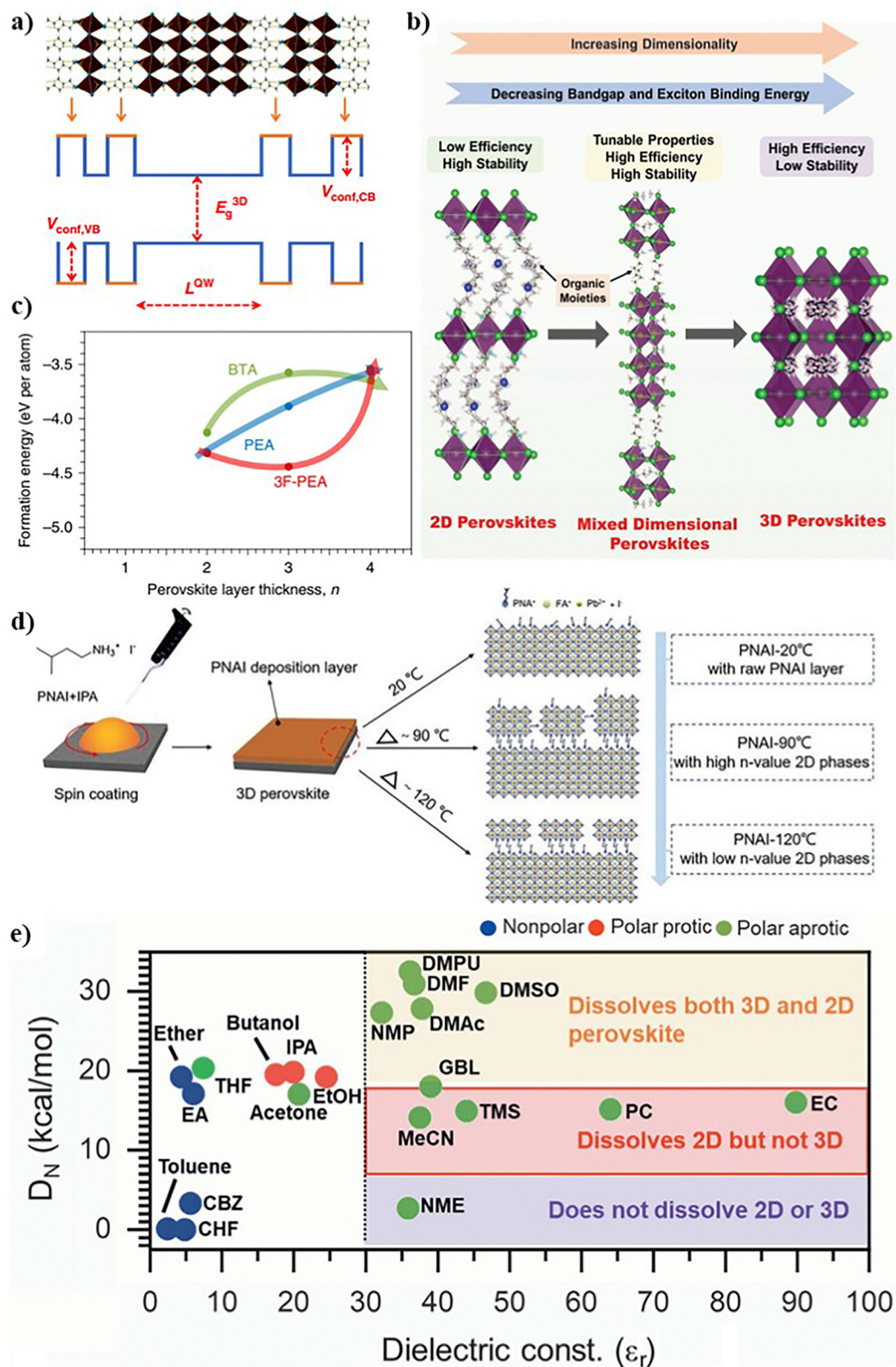
Fig. 4 (a) Schematic of a 2D/3D perovskite structure and possible energy-level schemes that can arise within these structures, where semiconducting inorganic sheets alternate with organic layers having much wider bandgaps, resulting in a Type I quantum well structure. (b) Illustration of a 2D crystalline structure, mixed-dimensional 2D/3D perovskites, and 3D perovskites. (c) The formation energy of different RDPs dependent on the layer width n and the ligands (BTA, PEA and 3F-PEA). 30 (d) The fabrication processes using different interfacial treatments. 75 (e) Plot showing different solvents based on the dielectric constant and the Gutmann number to identify the differences in solubility of the 3D and 2D perovskite powders for making a 3D/2D bilayer stack. 76
