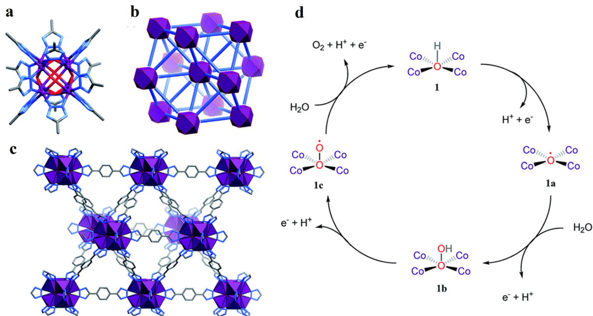
Fig. 12 (a) Co 8 (μ 4 -OH) 6 (Rtrz) 12 cluster (Rtrz - = 1,2,3-triazolate group), (b) network topology (octanuclear clusters: violet polyhedra and bistrizolate ligands: blue sticks), and (c) 3D coordination framework (CoN 3 O 3 units: violet polyhedra) of MAF-48 (hydrogen atoms are omitted for clarity). (d) Proposed reaction mechanism for using MAF-48 as CAT for light-driven water oxidation. Adapted with permission from ref. 165. Copyright 2019, the Royal Society of Chemistry.
