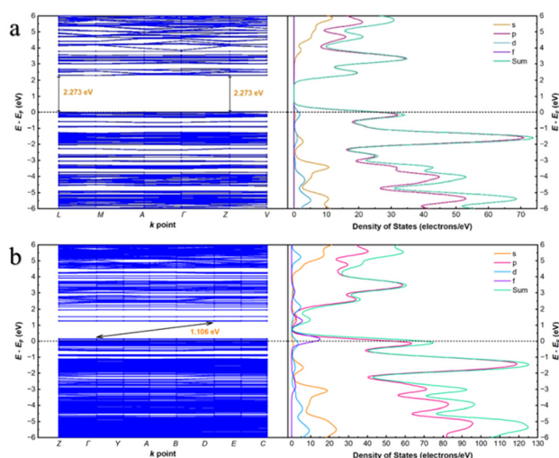
Fig. 9 Band structure versus PDOS of the Cd-MOF (a) and the \text{UO}_2^{2+}@\text{Cd-MOF} (b).
