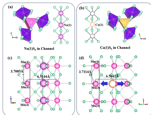
Fig. 5 Distribution of A-site cations in channels of NaMn 3 Ga 3 S 8 and CaMn 6 Ga 6 S 16 .
