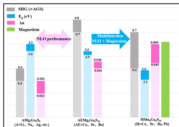
Fig. 6 Performance changes of A(l)B 3 C 3 S 8 and (AE/M)Mg 6 Ga 6 S 16 after element substitution.
