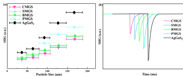
Fig. 4 (a) Phase-matching results of MMn 6 Ga 6 S 16 (M = Ca, Sr, Ba, and Pb) and the benchmark AGS at 2090 nm and (b) SHG intensities of MMn 6 Ga 6 S 16 (M = Ca, Sr, Ba, and Pb) and AGS with the particle size ranging from 150–200 μm.
