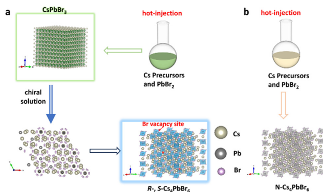
Fig. 1 (a) Schematic of the phase transformation from 3D cubic \text{CsPbBr}_3 to hexagonal 0D R - and S - \text{Cs}_4\text{PbBr}_6 NCs. (b) Schematic of the synthesis of N- \text{Cs}_4\text{PbBr}_6 NCs.
