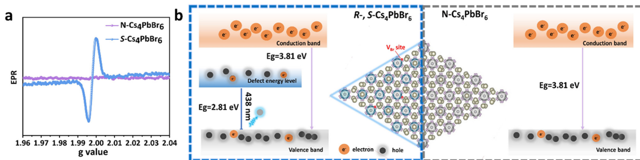
Fig. 5 (a) EPR spectra of S-Cs 4 PbBr 6 NCs and N-Cs 4 PbBr 6 NCs. (b) Schematic of the comparison of electronic band structure and luminescence mechanism for chiral Cs 4 PbBr 6 NCs (left) and N-Cs 4 PbBr 6 NCs (right).
