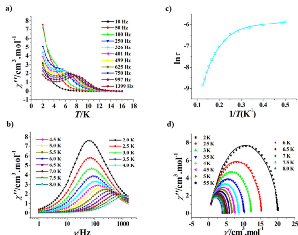
Fig. 6 Plots of \chi'' versus T for D-1 ( H_{\text{dc}} = 0 \text{ Oe} ) (a). Frequency dependence of \chi'' for D-1 at a zero dc field (b). Plot of \ln(\tau) versus 1/T for D-1 ( H_{\text{dc}} = 0 \text{ Oe} ); the solid line represents the best fitting with quantum tunnelling plus Orbach plus Raman (c). Cole–Cole plots measured from 2.0 to 8.0 K for D-1 ( H_{\text{dc}} = 0 \text{ Oe} ); the solid lines represent the best fitting with the generalized Debye model (d).
