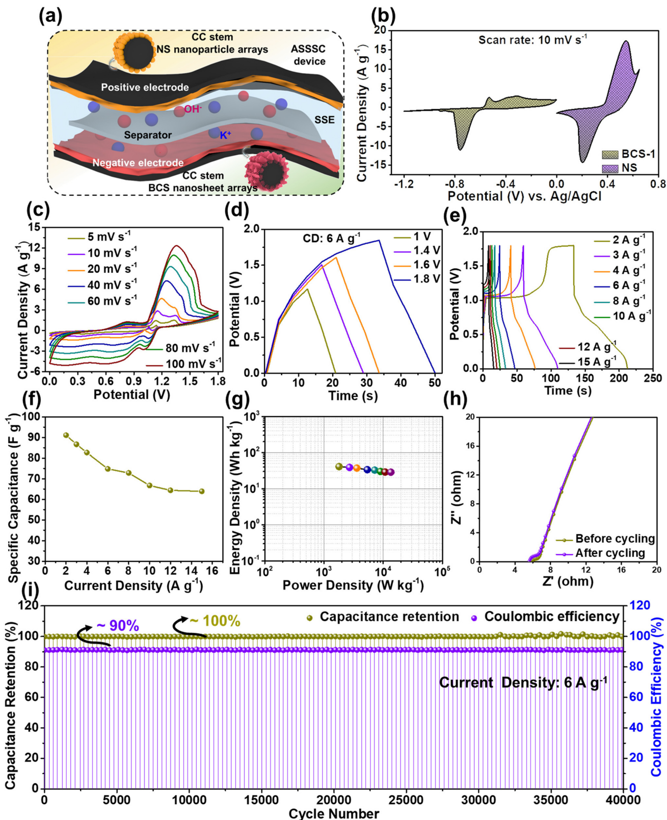
Fig. 6 (a) A schematic illustration of the as-assembled AS SSC device. (b) Merged CV plots of the NS and BCS-1 electrodes measured in a three-electrode system, (c) CV curves at different scan rates with the optimized OPW, (d) GCD curves at different potentials for optimization, and (e) GCD curves at different current densities with the optimized OPW for the AS SSC device. (f) C_s values vs. various current densities, (g) Ragone plot, (h) EIS plots before and after the cycling test, and (i) cycling stability performance for the AS SSC device.
