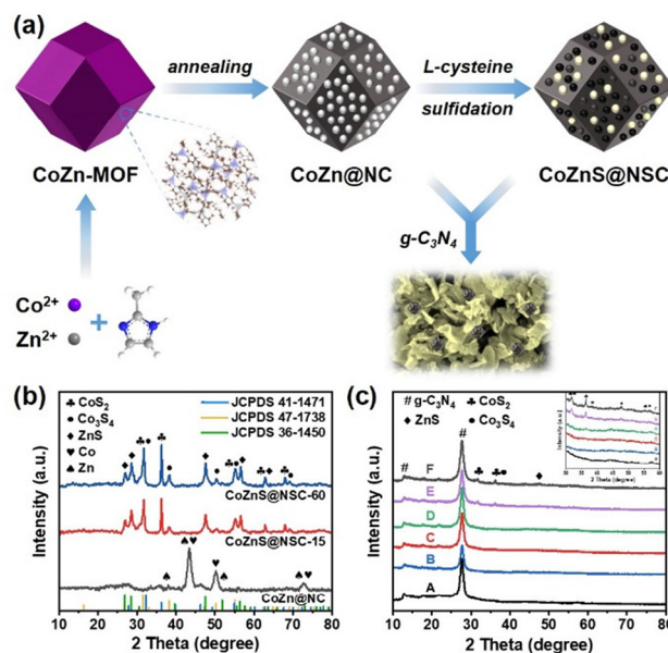
Fig. 1 (a) Schematic diagram of the synthesis of CoZn-MOF, CoZn@NC, CoZn@NC/g-C 3 N 4 , CoZnS@NSC, and CoZnS@NSC-X/g-C 3 N 4 samples. XRD patterns of (b) CoZn@NC, CoZnS@NSC-15, and CoZnS@NSC-60 nanoparticles and (c) g-C 3 N 4 (A), CoZn@NC/g-C 3 N 4 (B), and CoZnS@NSC/g-C 3 N 4 after sulfidation for 15 (C), 30 (D), 45 (E), and 60 min (F).
