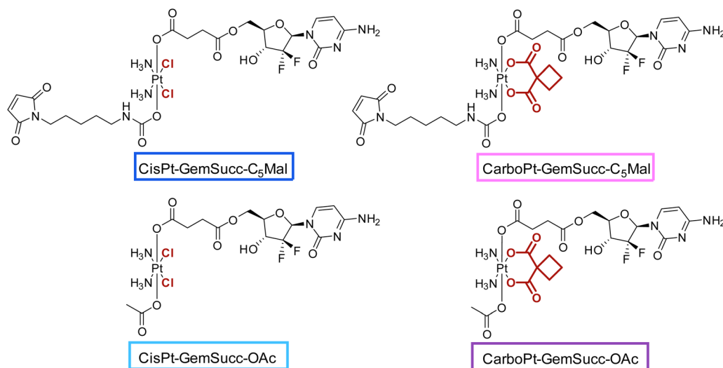
Fig. 7 Third panel of maleimide-platinum( iv )-gemcitabine complexes, with two different platinum core structures (cisplatin vs. carboplatin).
