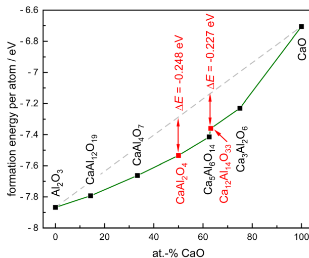
Fig. 7 Convex-hull diagram (formation energy per atom versus chemical composition) for the ternary system Ca–Al–O with respect to the binary oxides CaO and \text{Al}_2\text{O}_3 . The formation energy per atom is obtained from DFT calculations.
